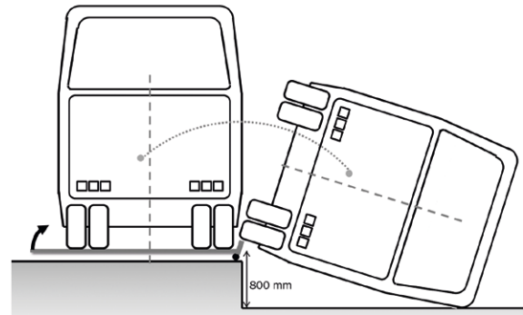
D: Rollover test 2
