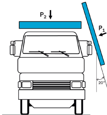
C: Roof strength 1
