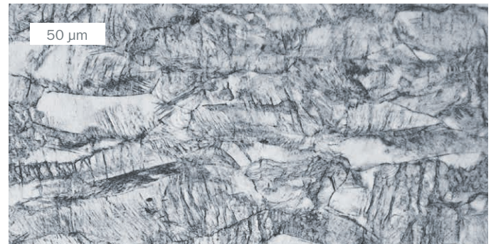
56.8 % strain-hardening
