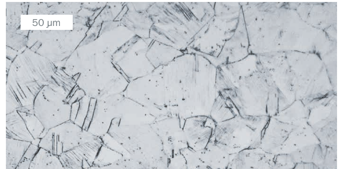
13.6 % strain-hardening
